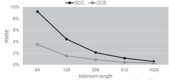
Figure 7: Average RMSE of a 3 \times 3 Gaussian blur filter when following the alignment recommended by SCC and ZCE.
