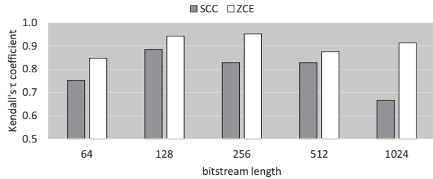
Figure 10: Kendall's \tau coefficient of the rankings produced by ZCE and SCC for a 3 \times 3 Gaussian blur benchmark.
