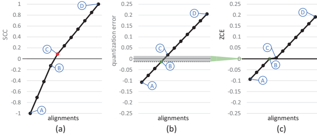
Figure 4: Plots of (a) SCC, (b) true error and (c) ZCE for all possible alignments of P_X \times P_Y = \frac{21}{32} \times \frac{22}{32} . Point B is the most independent alignment, whereas SCC incorrectly identifies point C as the most independent alignment.
