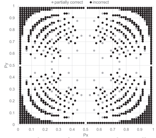
Figure 3: Distribution of incorrect and partially correct alignments for independence identified by SCC, for a bitstream length of 64. The horizontal and vertical axes show the values represented by two SC bitstreams P_X and P_Y , respectively. Black dots indicate combinations of P_X, P_Y values where SCC incorrectly identifies the maximally independent alignment. Grey dots indicate combinations of P_X, P_Y values where SCC only identifies one of the maximally independent alignments.
