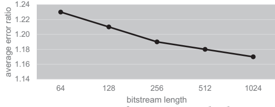
Figure 5: Average error of AND-gate multiplication when following the alignment recommended by SCC, normalized to quantization error.
