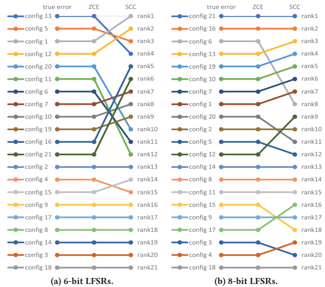
Figure 9: Ranking of 6-bit and 8-bit LFSR configurations based on true error (via AND-gate multiplication), ZCE and SCC, averaged over all possible input value pairs. ZCE’s and SCC’s rankings yield a Kendall’s \tau coefficient of 1 and 0.82 respectively for 6-bit LFSRs, and 1 and 0.83 for 8-bit LFSRs.
