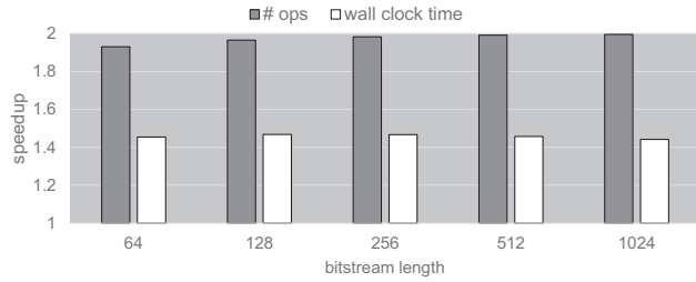
Figure 8: Speedup of using ZCE to determine whether bitstreams are optimally aligned compared to using SCC.
