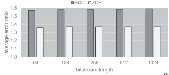
Figure 6: Average error of scale-by-4 addition ( P_Z = \frac{P_X + P_Y}{4} ) when following the alignment recommended by SCC and ZCE, normalized to quantization error.
