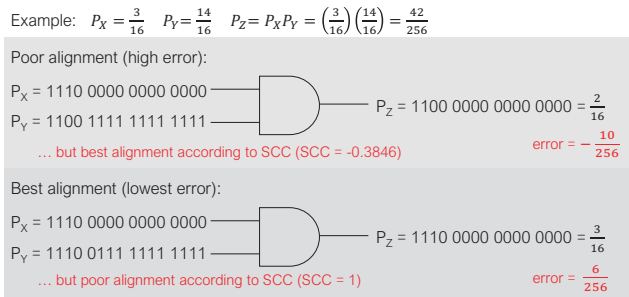
Figure 1: Example of when an alignment with the lowest |SCC| does not correspond to the one with highest accuracy.
