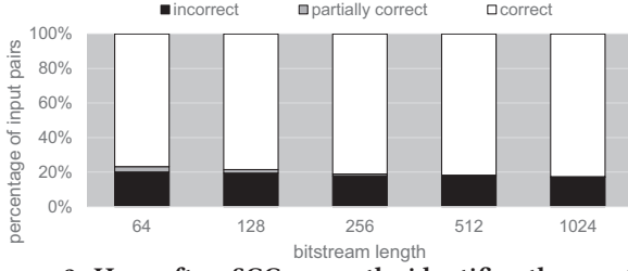
Figure 2: How often SCC identifies the most independent input pairs. Correct refers to when SCC identifies the same alignment as the maximally independent alignment; partially correct refers to when SCC identifies the same alignment as one of the maximally independent alignments (i.e. when two alignments have the same |P_{X \wedge Y} - P_X P_Y| ); and incorrect refers to when SCC identifies a different alignment from the maximally independent one.
